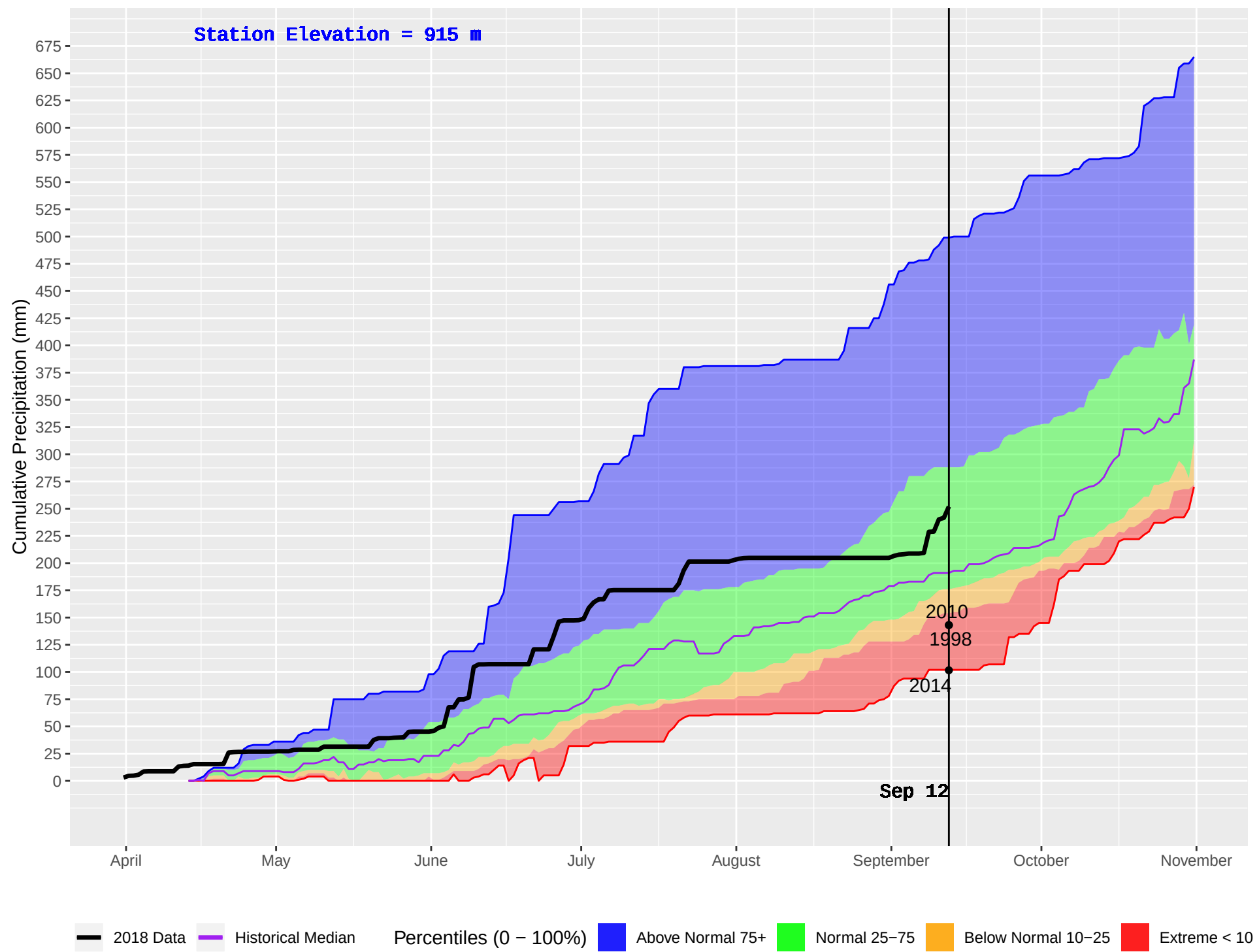
MCLEOD LAKE (153) : Historical (1990–2016) and Current (2018) Daily Cumulative Precipitation
