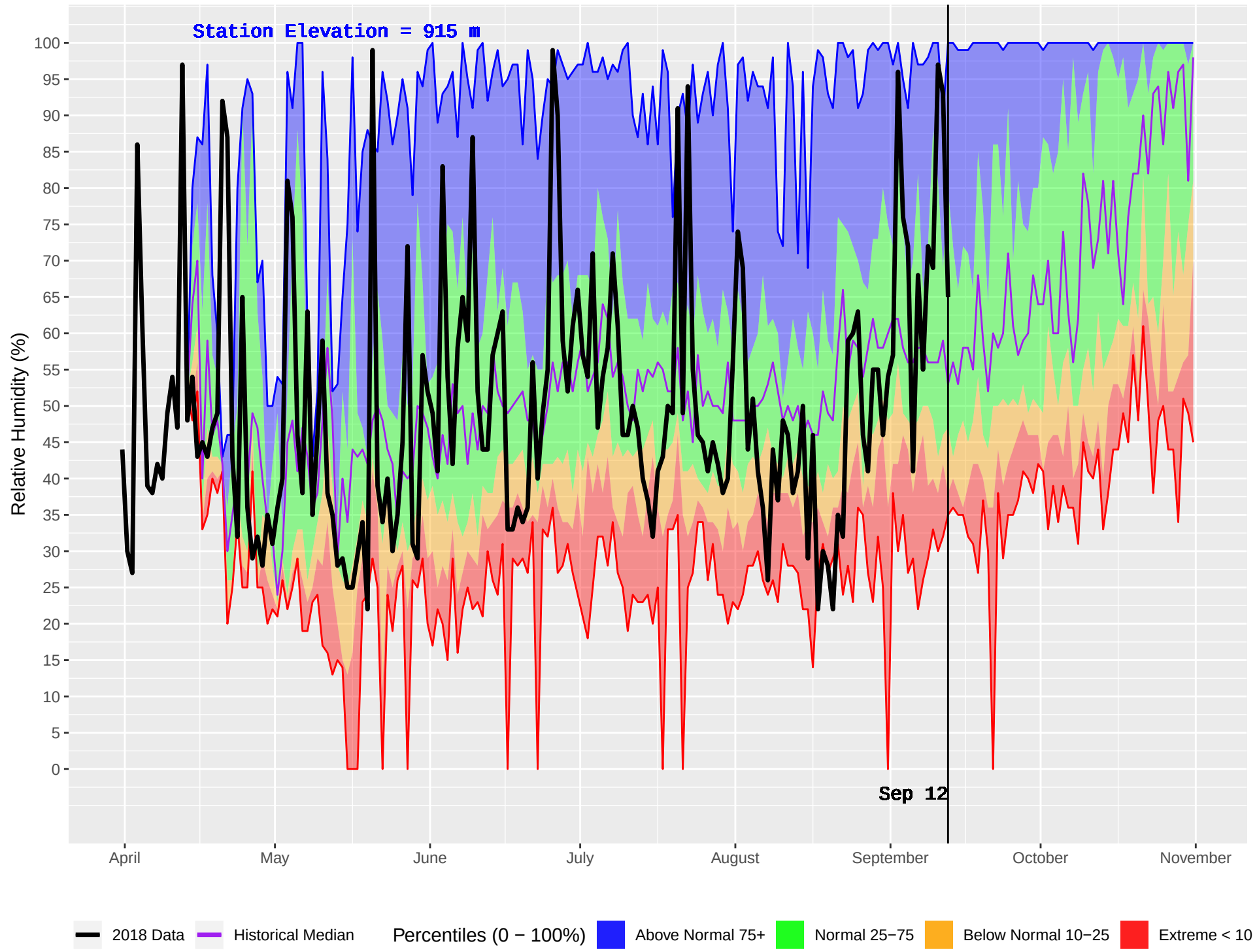
MCLEOD LAKE (153) : Historical (1990–2016) and Current (2018) Daily Relative Humidity
