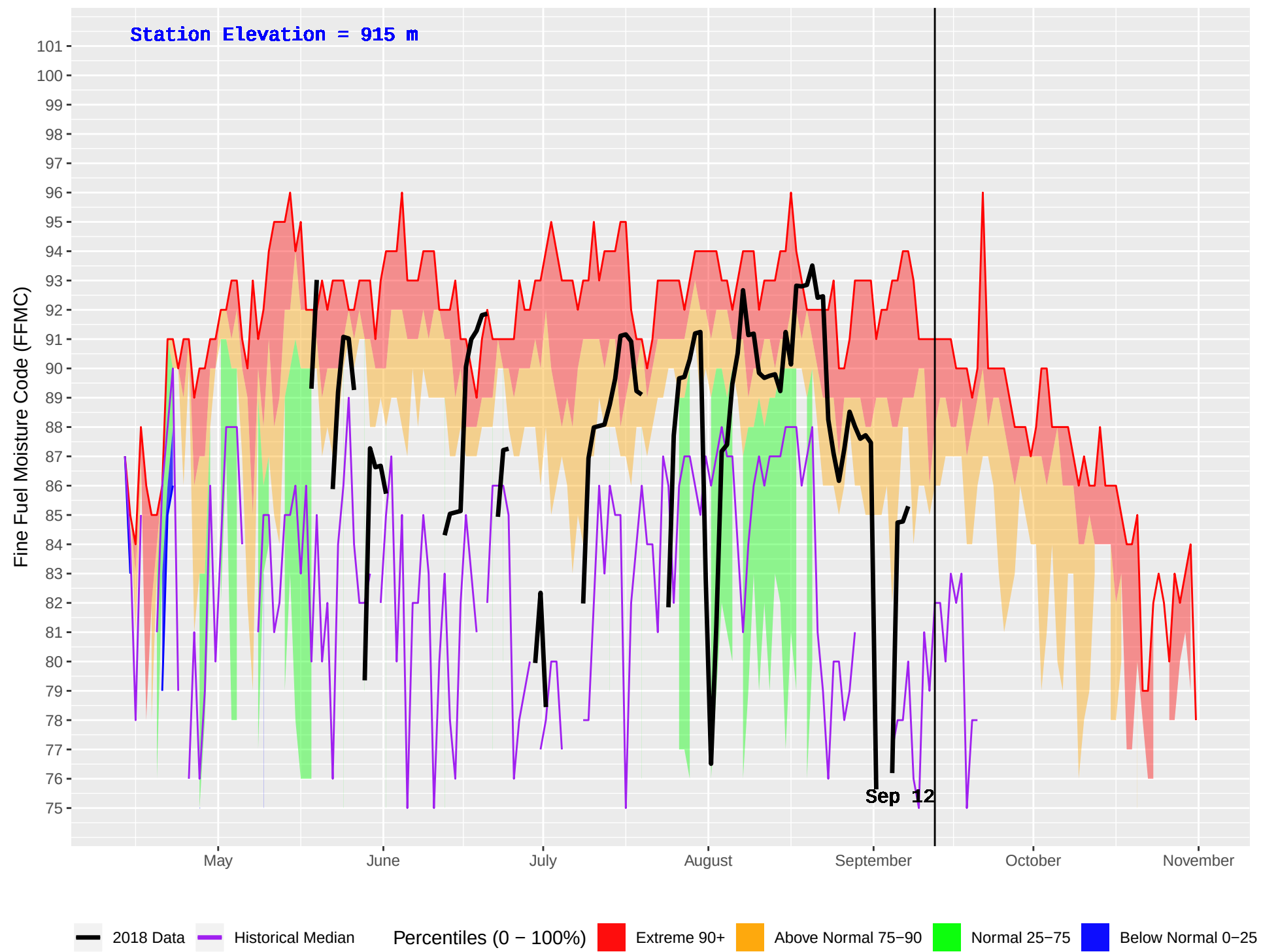
MCLEOD LAKE (153) : Historical (1990–2016) and Current (2018) Daily Fine Fuel Moisture Code (FFMC)
