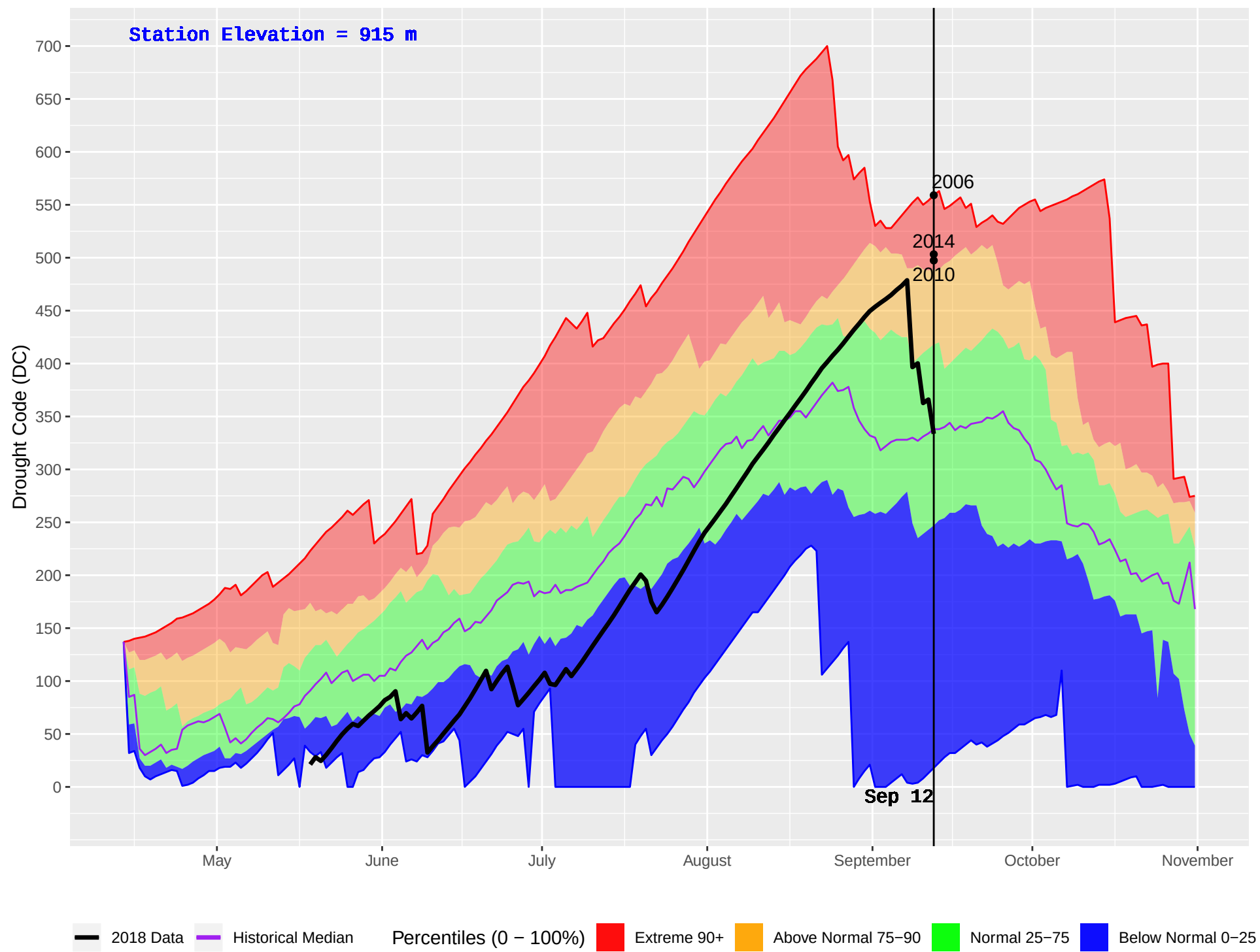
MCLEOD LAKE (153) : Historical (1990–2016) and Current (2018) Daily Drought Code (DC)
