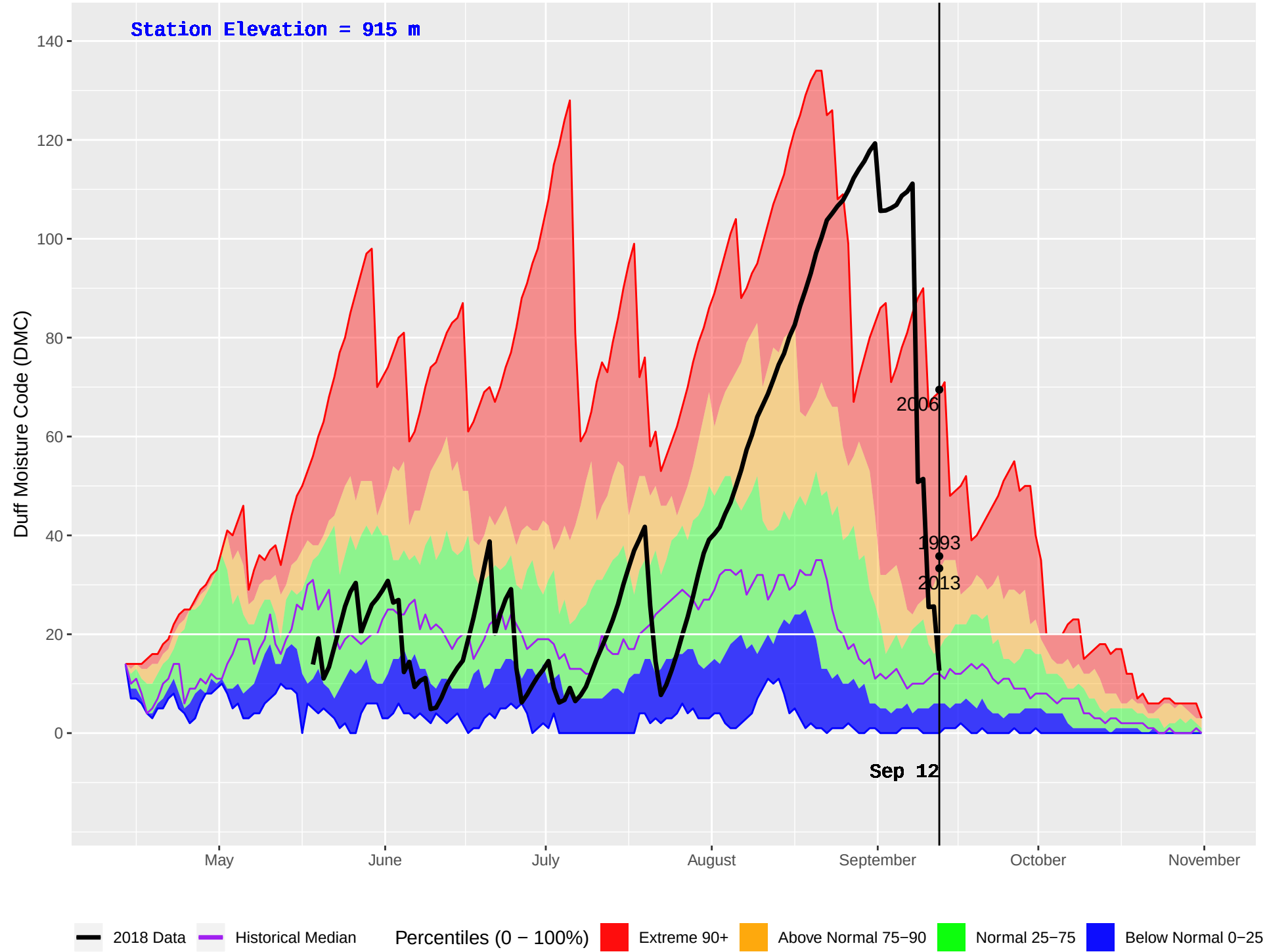
MCLEOD LAKE (153) : Historical (1990–2016) and Current (2018) Daily Duff Moisture Code (DMC)
