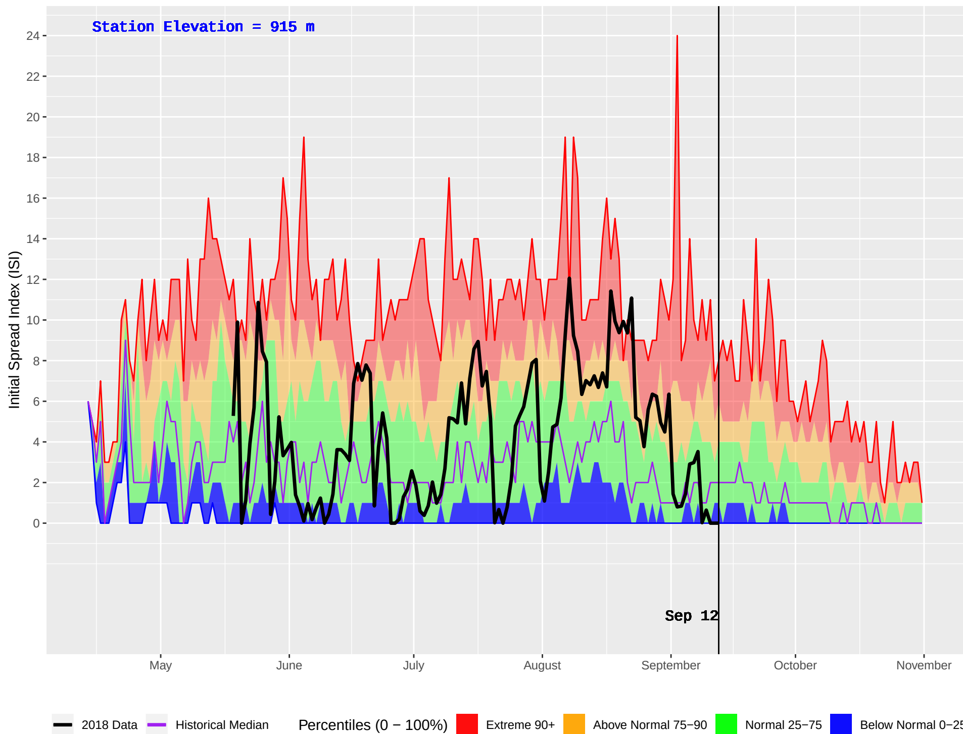
MCLEOD LAKE (153) : Historical (1990–2016) and Current (2018) Daily Initial Spread Index (ISI)
