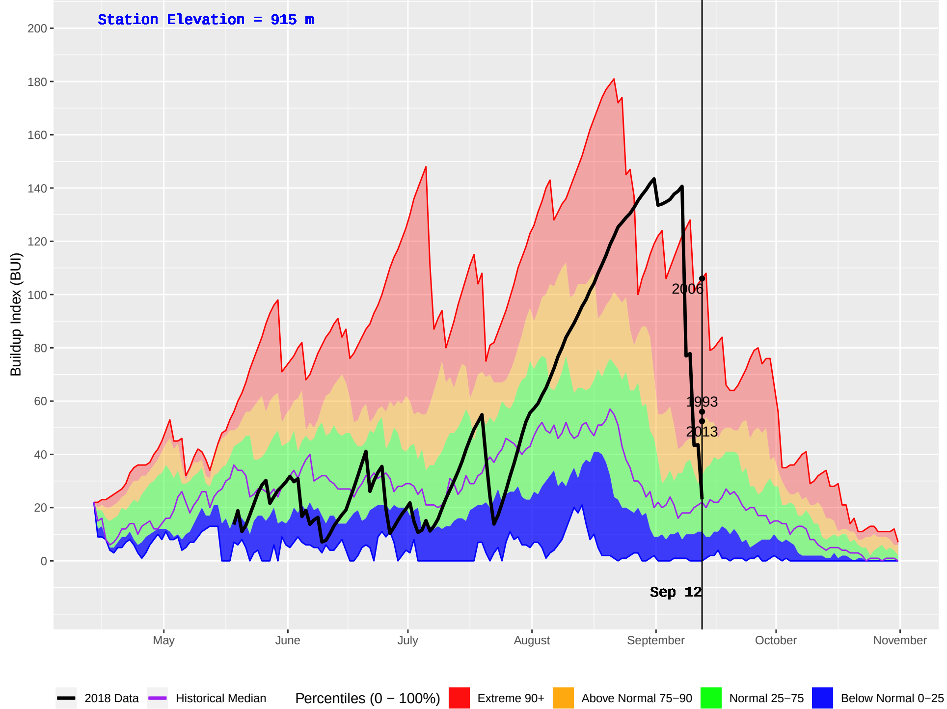
MCLEOD LAKE (153) : Historical (1990–2016) and Current (2018) Daily Buildup Index (BUI)
